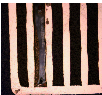
Fig. 15. Vectors with 72.5 Watt power and 80 μs laser exposure time
