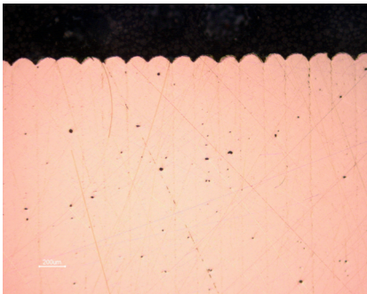
Fig. 21. Cross section of the vectors with 180 µm distance
