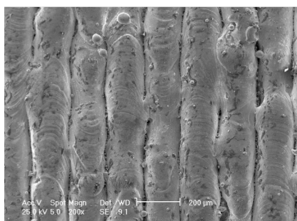
Fig. 32. Single laser scan on the gallium containing alloy. Porosity is present. SEM image
