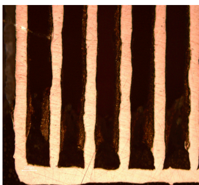
Fig. 16. Vectors with 62.5 Watt power and 80 μs laser exposure time
