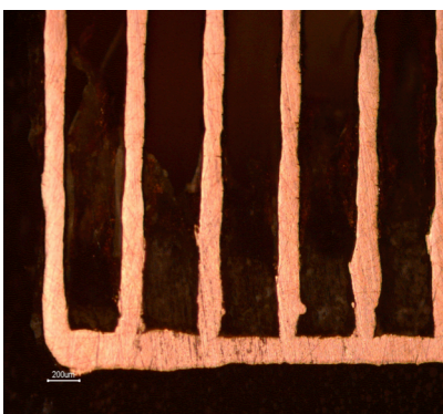
Fig. 12. Vectors with 62.5 Watt power and 0.5 m/s scanning speed
