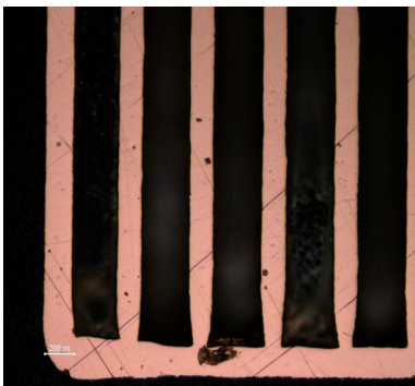
Fig. 8. Vectors with 62.5 Watt power
