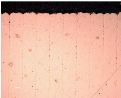
Fig. 20. Cross section of the vectors with 160 µm distance
