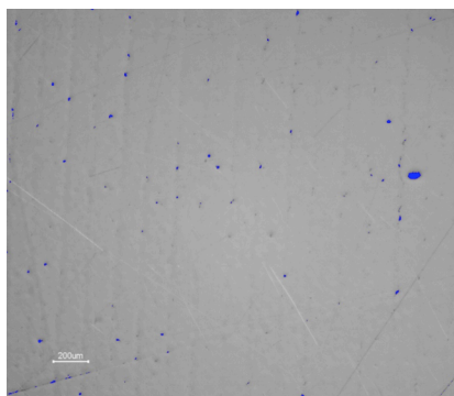
Fig. 28. Example of a digital porosity analysis for a standard alloy (2)
