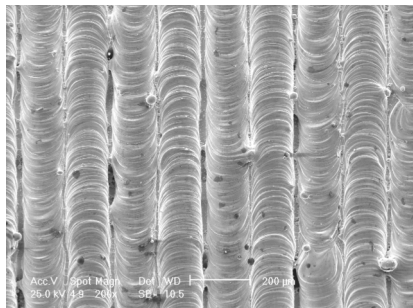
Fig. 27. SEM image after a typical double scan
