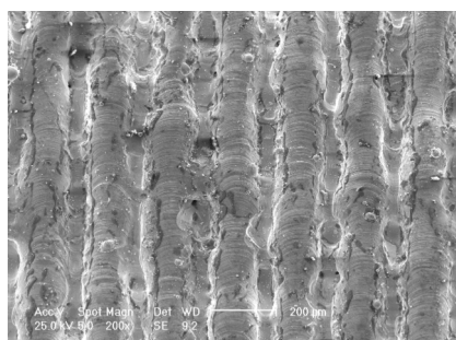
Fig. 31. Double laser scan between the vectors on the gallium containing alloy. SEM image
