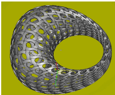
Fig. 46. Tri-dimensional model of the ring with parametric texture obtained with Magics (Materialise)
