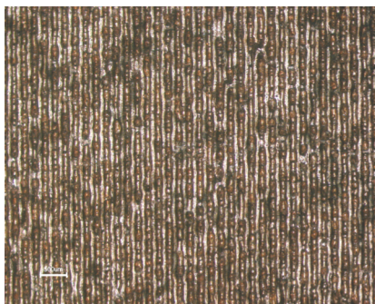
Fig. 29. Surface after double laser scan, gallium containing alloy
