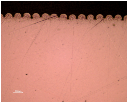
Fig. 40. SLM - Powder with 5-53 µm particle size range
