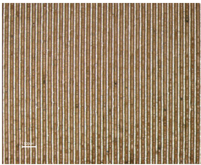
Fig. 24. Upper surface after double laser scan
