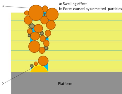
Fig. 35. Final stage of laser melting with formation of porosity and swelling
