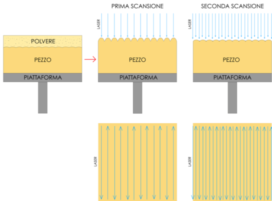
Fig. 23. Schematic representation of a double laser scan
