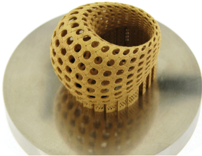
Fig. 47. Ring with parametric texture after completion of the production
