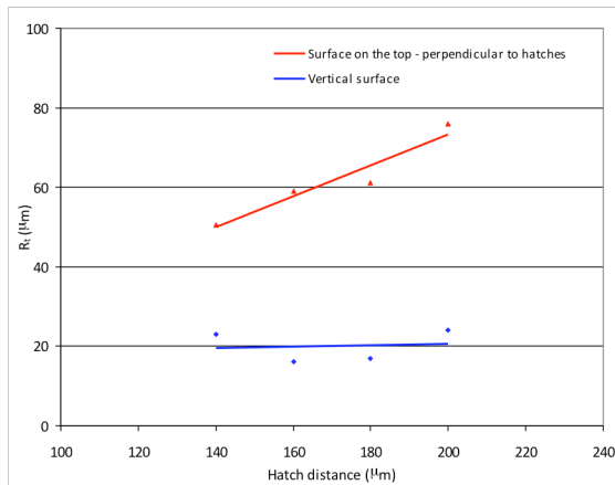
Fig. 18. Roughness R_f as a function of the distance between the vectors on the faces of the solid piece
