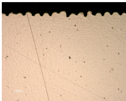
Fig. 30. — Metallographic cross section after double laser scan, gallium containing alloy
