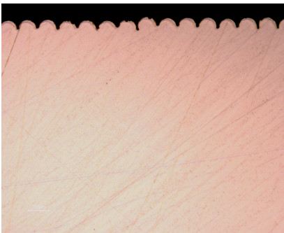
Fig. 25. Metallographic section of the piece with double laser scan
