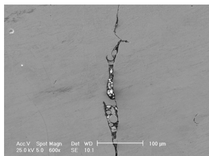
Fig. 33. Build-up of pores and particle clusters in the zone between the vectors
