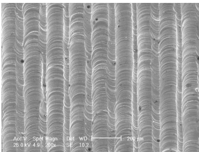
Fig. 26. SEM image before the second scan, with porosity
